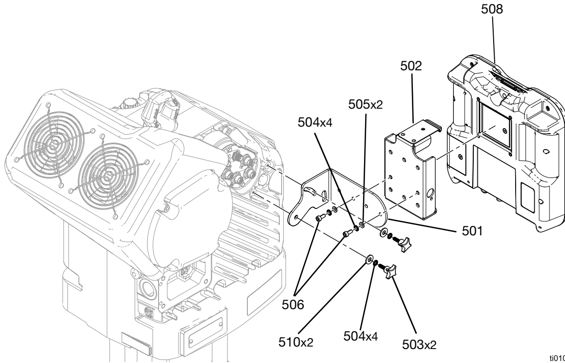
FIG. 21: ADM Kit
