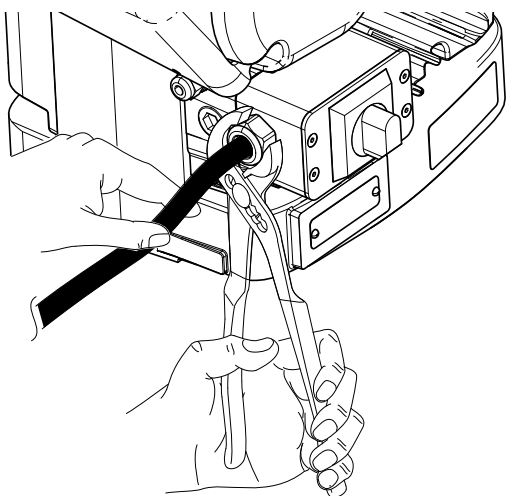
FIG. 7: Tighten Cord Grip
