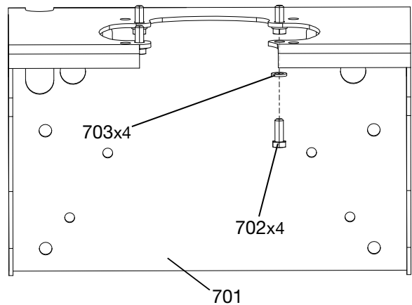
FIG. 28: Wall Mount Bracket
