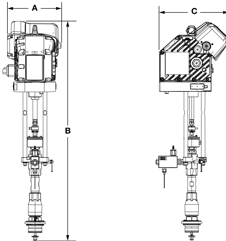
FIG. 31: 220 cc Dura-Flo CS Pump System Dimensions
