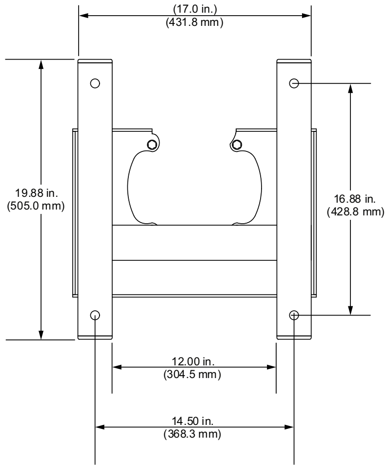
FIG. 32: Pump Stand Mounting Holes
