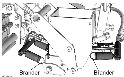
FlexDiebrander (ThermoLazer 200/200TC)
