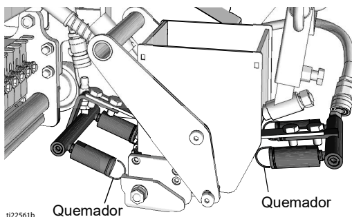
FlexDie Quemador (ThermoLazer 200/200tc)
