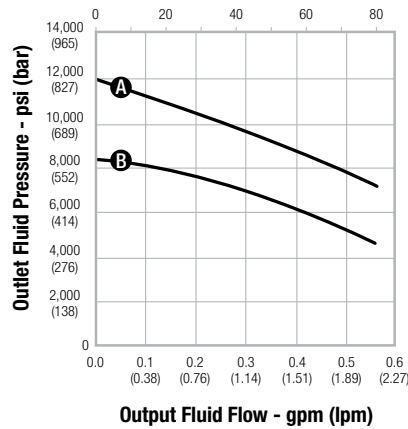
Dyna-Star 120:1 Pump Performance Curve Air Motor Speed — CPM
