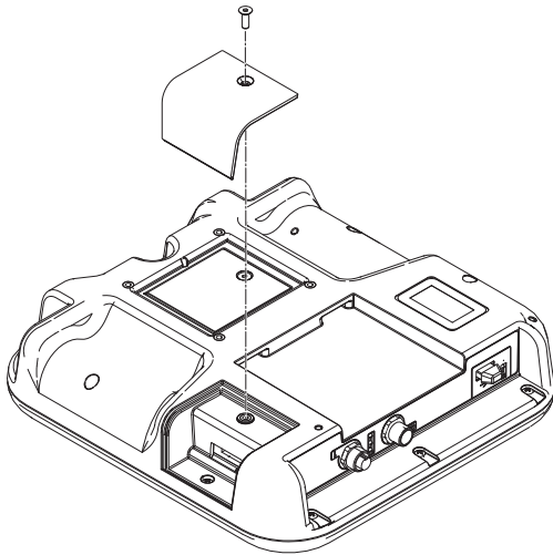
FIG. 2: Remove Token Access Cover
