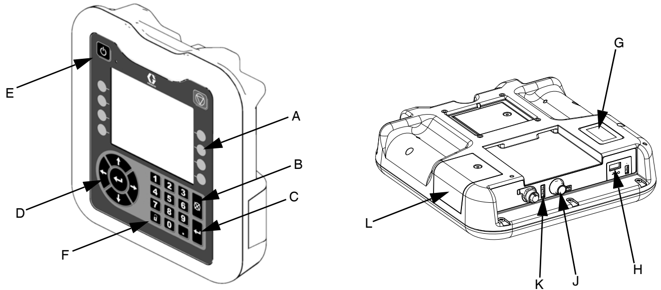
FIG. 1: ADM Component Identification - Front and Rear Views
