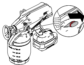
Trigger Unlocked (red ring is visible)
