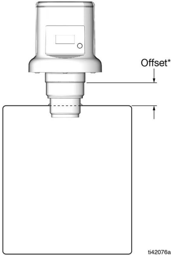
FIG. 16: NOTE: *TLM Offset is the distance from the maximum height to the shoulder above the threads on TLM.
