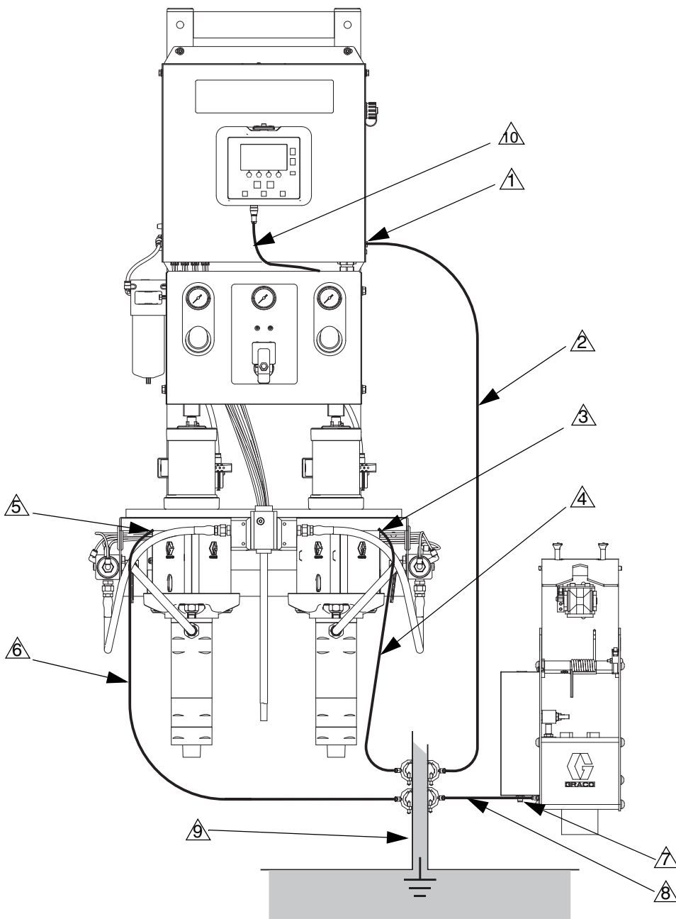
AFB. 9. Aarding
