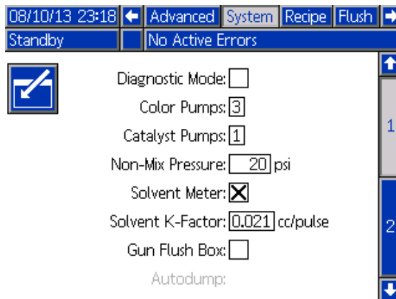
Figure 15 Systembildschirm 1
