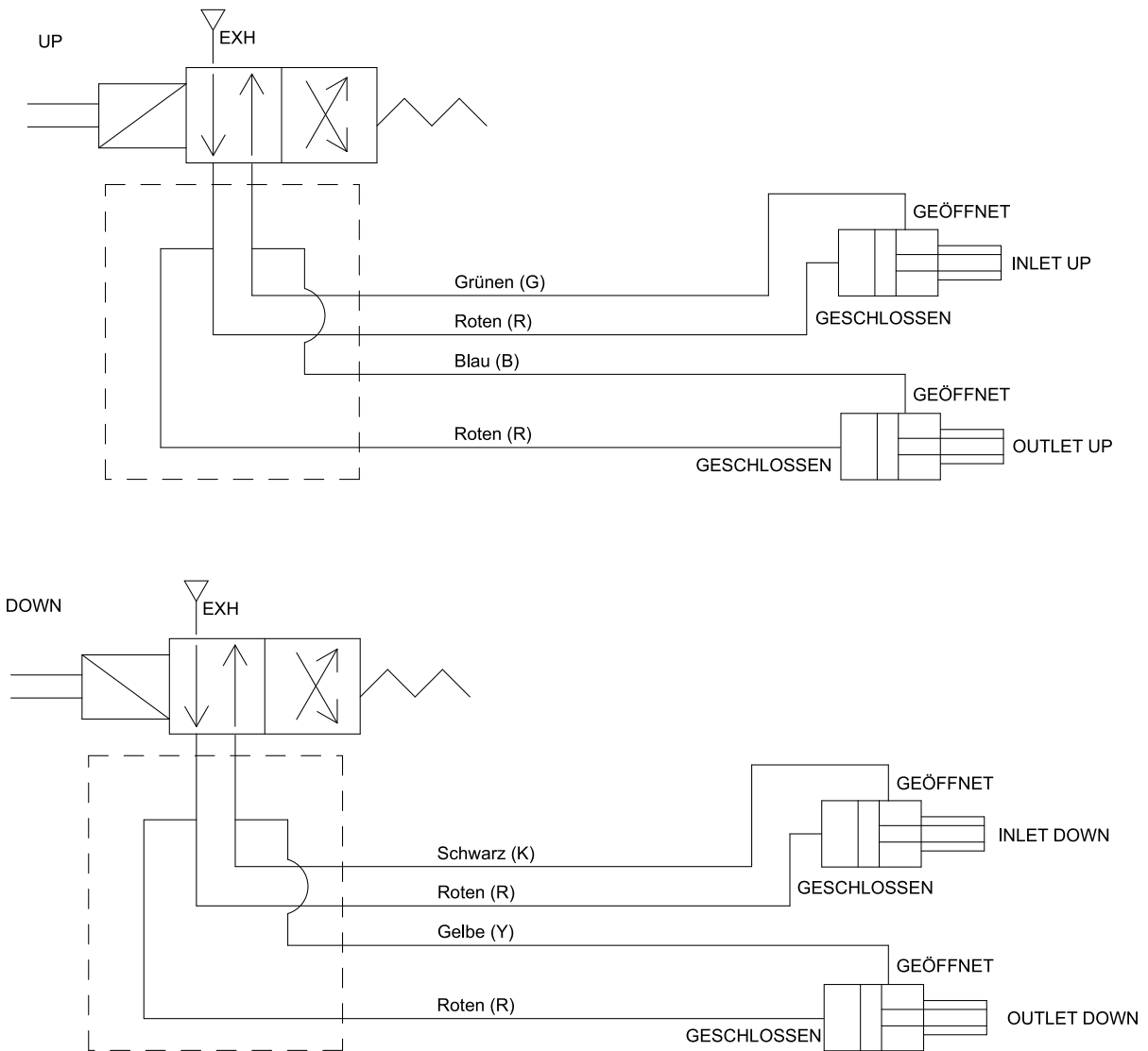
Figure 23 Pumpenschlauchschemata
